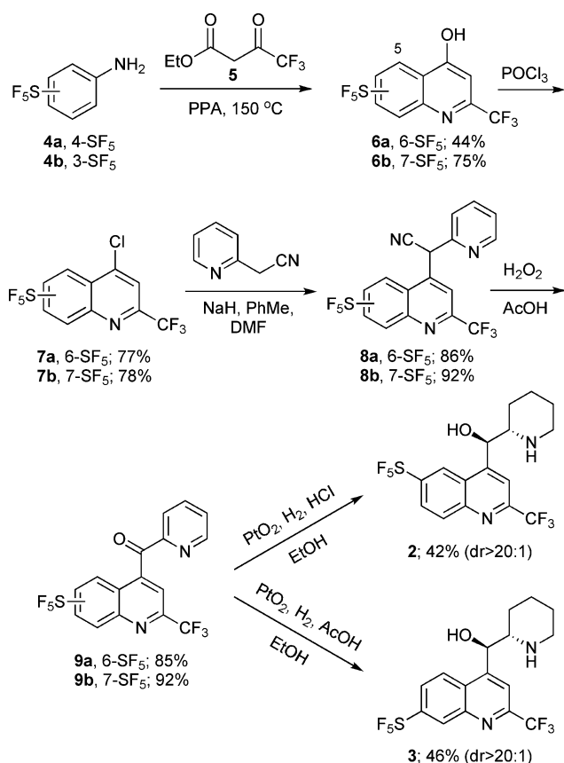
Scheme 1 Synthesis of mefloquine analogs 2 and 3 .
