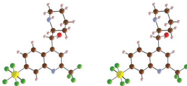
Fig. 3 Stereoview of the X-ray structure of 3 .
