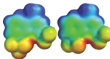
Fig. 2 Electron-density surfaces/electrostatic potential maps calculated with Spartan 08 (HF/6–31G*) for 2 analogs of 1, 4-methyl-8-pentafluorosulfanyl-2-trifluoromethylquinoline (left) and 4-methyl-2,8-bis(trifluoromethyl)quinoline (right).
